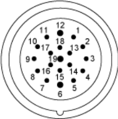
M23 Connector
